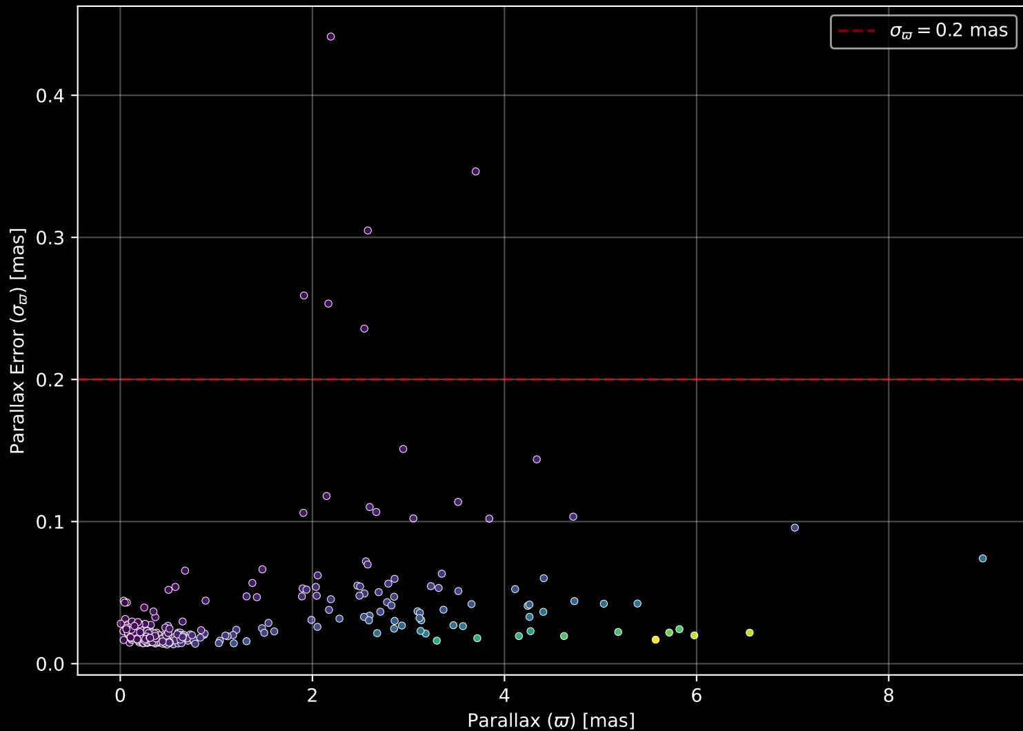
APOGEE DR17 Field: [140-18_btx] Parallax Quality (n= 310)
