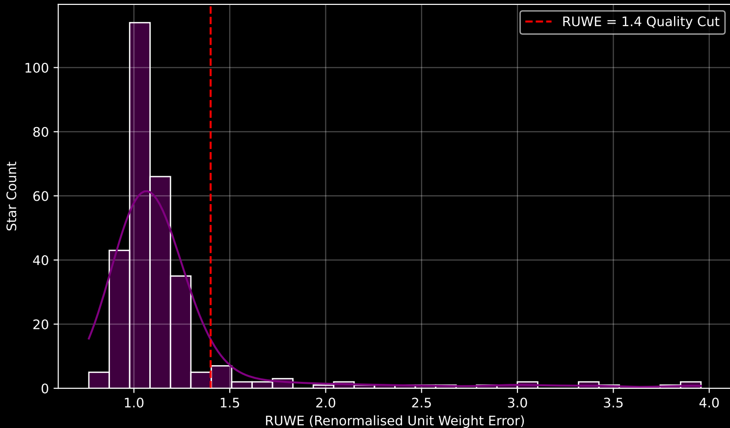
GAPOGEE DR17 Field [140-18_btx] RUWE Distribution (n= 300)
