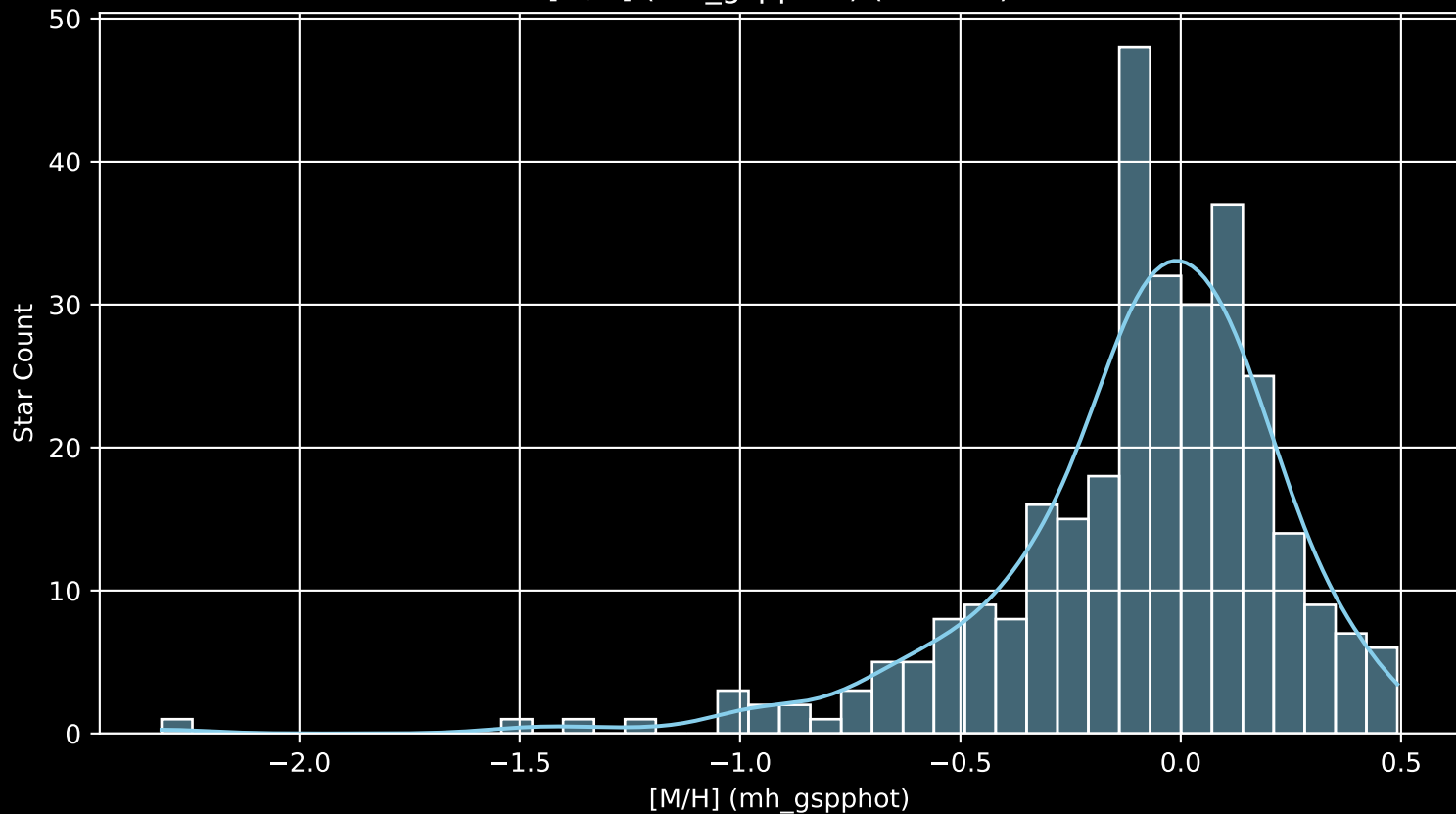
APOGEE DR17 Field: [140-18_btx [M/H] (mh_gspphot) (n= 307)
