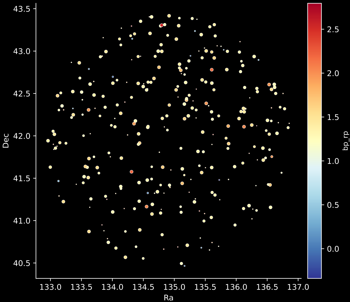
APOGEE DR17 Field: [140-18_btx] Stars: 310
