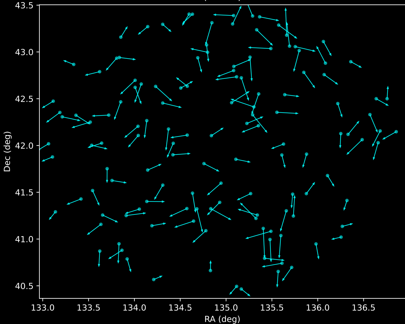
APOGEE DR17 Noise Stream Proper Motion Vectors (n=132)
