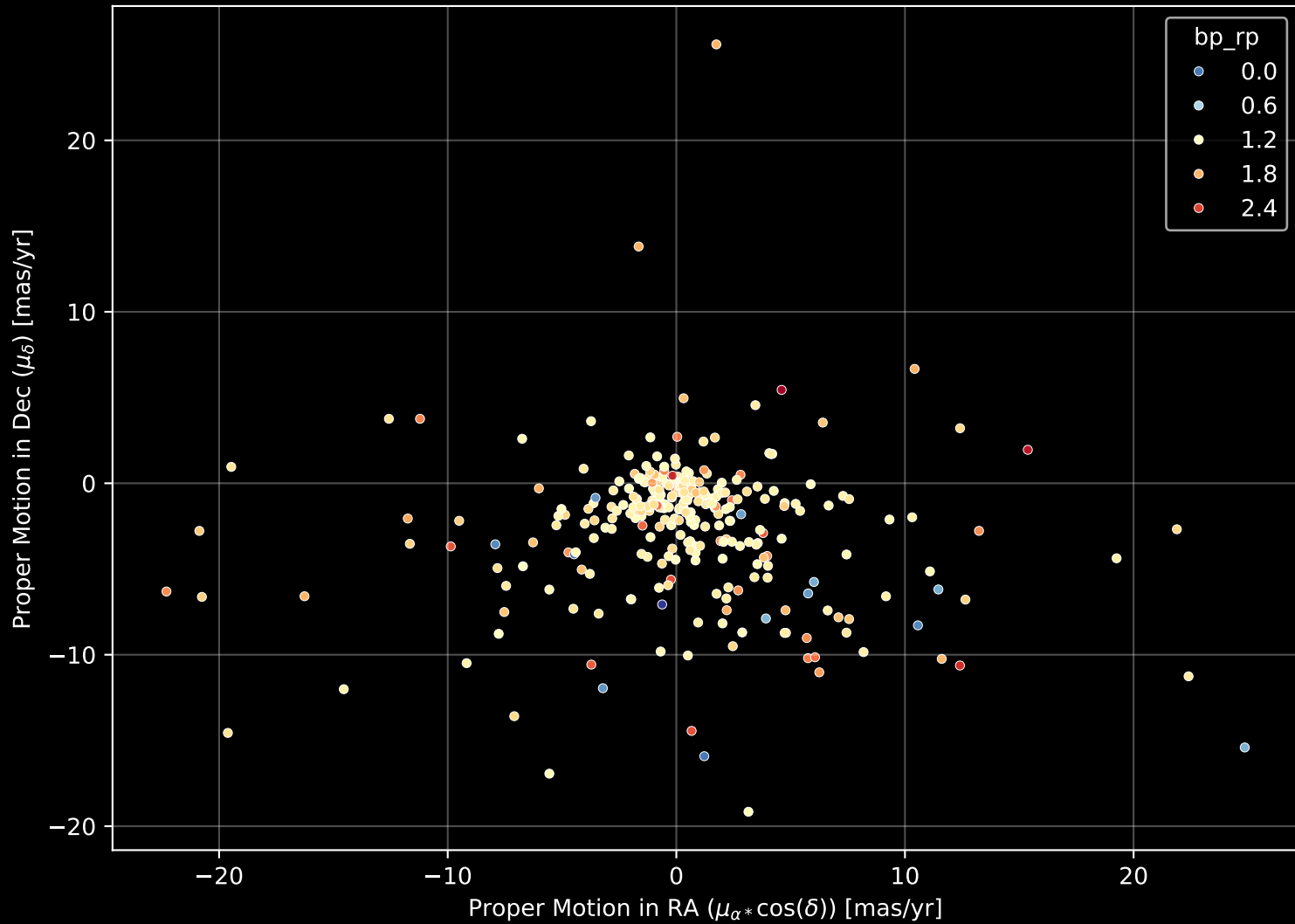
APOGEE DR17 Field: [140-18_btx] Proper Motion Diagram (n= 310)
