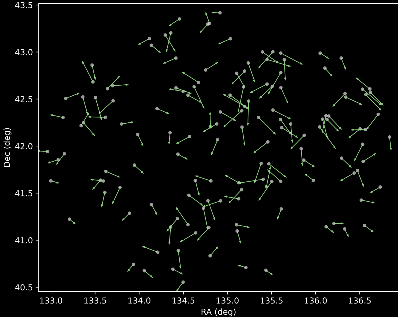
APOGEE DR17 Cluster 5 Proper Motion Vectors (n=140)
